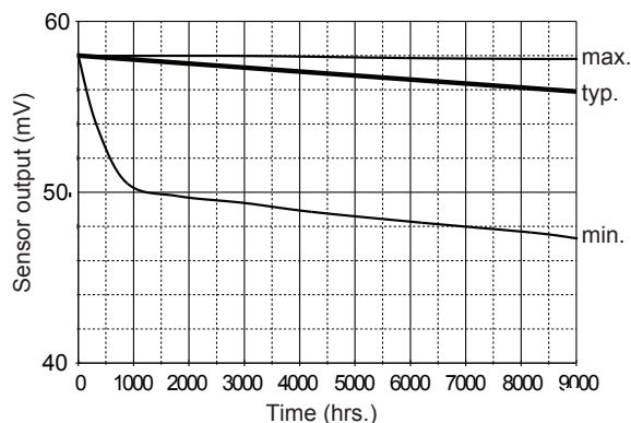
Fig. 10b - KE-50 long term stability
